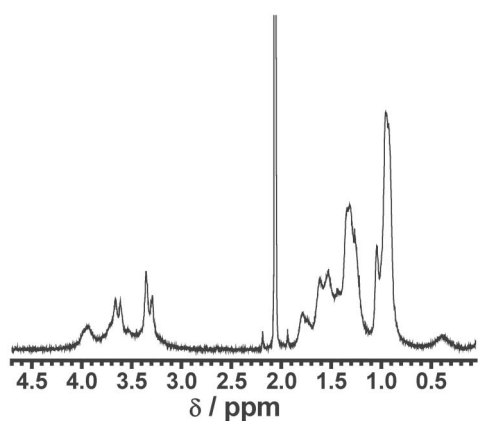
Fig. 4. 500 MHz ^1\text{H} NMR spectra of a 0.5% solution of MEH-PPV in \text{C}_6\text{D}_5\text{CD}_3 at -20\text{ }^{\circ}\text{C} . The band at 0.4 ppm is much broader and its intensity has been significantly diminished relative to that of the room temperature spectra ( vide Fig. 1).
